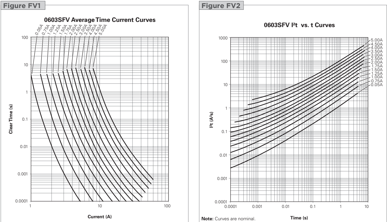
Figures FV1-FV2 Family Performance Curves for Very Fast-Acting Chip Fuses
