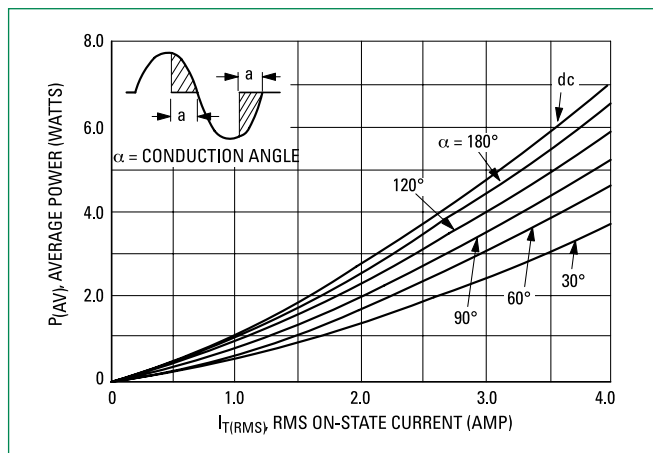
Figure 4. Power Dissipation
