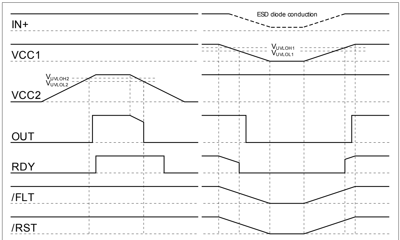
Figure 9 UVLO Behavior
