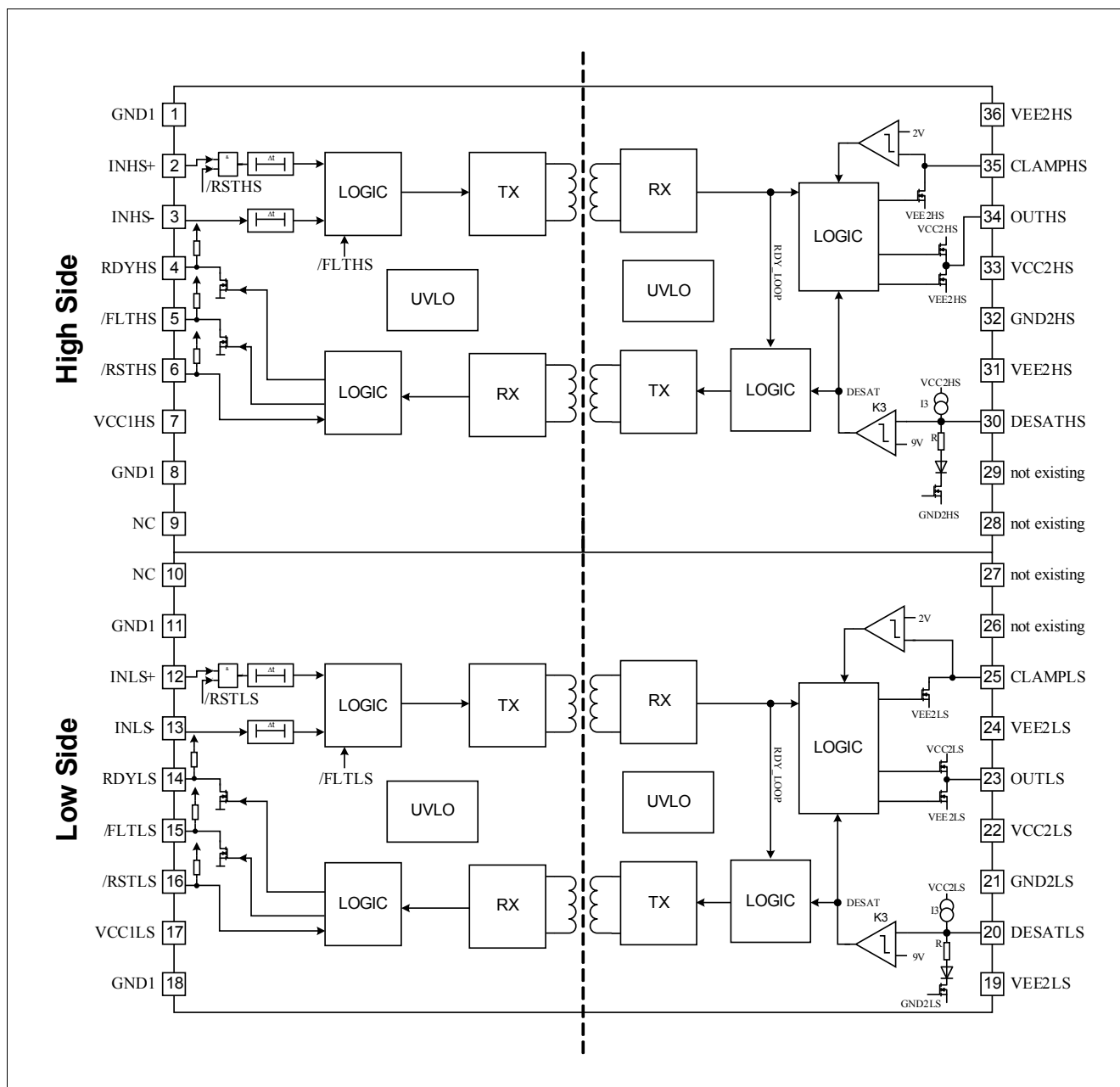
Figure 2 Block Diagram 2ED020I12-F2
