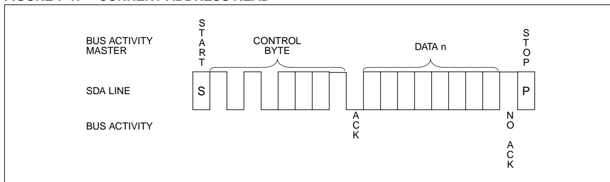
FIGURE 7-2: RANDOM READ
