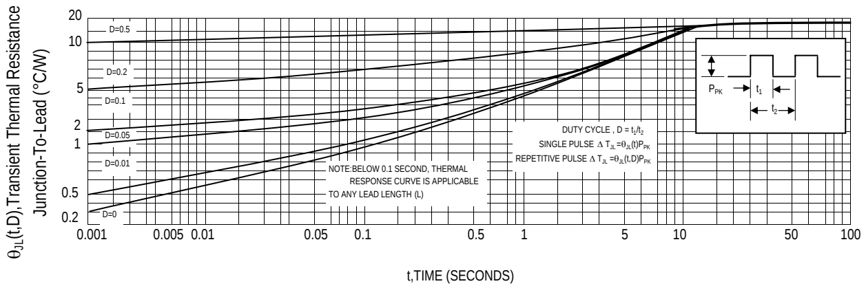
Fig 2. Typical Thermal Response L, Lead Length = 3/8 Inch
