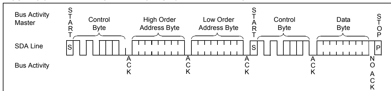
FIGURE 8-3: RANDOM READ: 32 TO 1024 KBIT DEVICES
