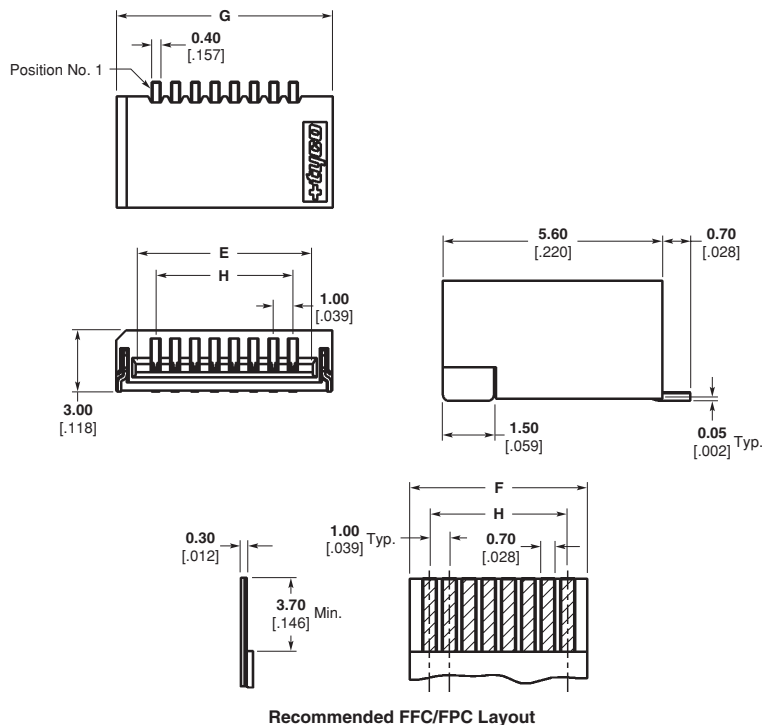
Recommended FFC/FPC Layout
