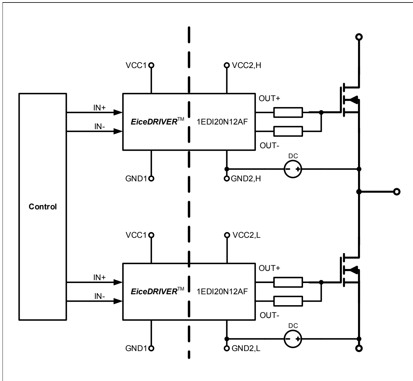
Figure 1 Typical Application
