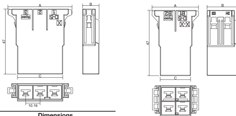
Panel/Free-hanging Type
