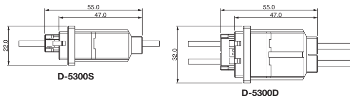
Panel/Free-hanging Type
