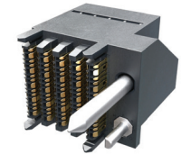
Right Angle Header (Left Guide)
