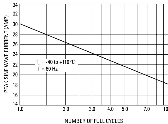
Figure 9. Maximum Allowable Surge Current
