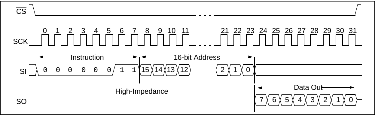
FIGURE 2-1: READ SEQUENCE
