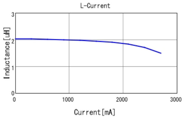
1231AS-H-2R2M L-Current 20degC
