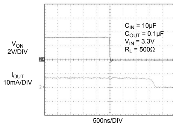
Figure 16. t_{dOFF} Response
