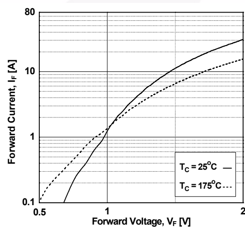
Figure 18. Forward Characteristics
