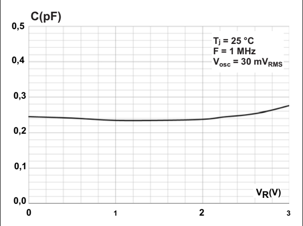
Figure 4. Junction capacitance versus applied voltage (typical values)
