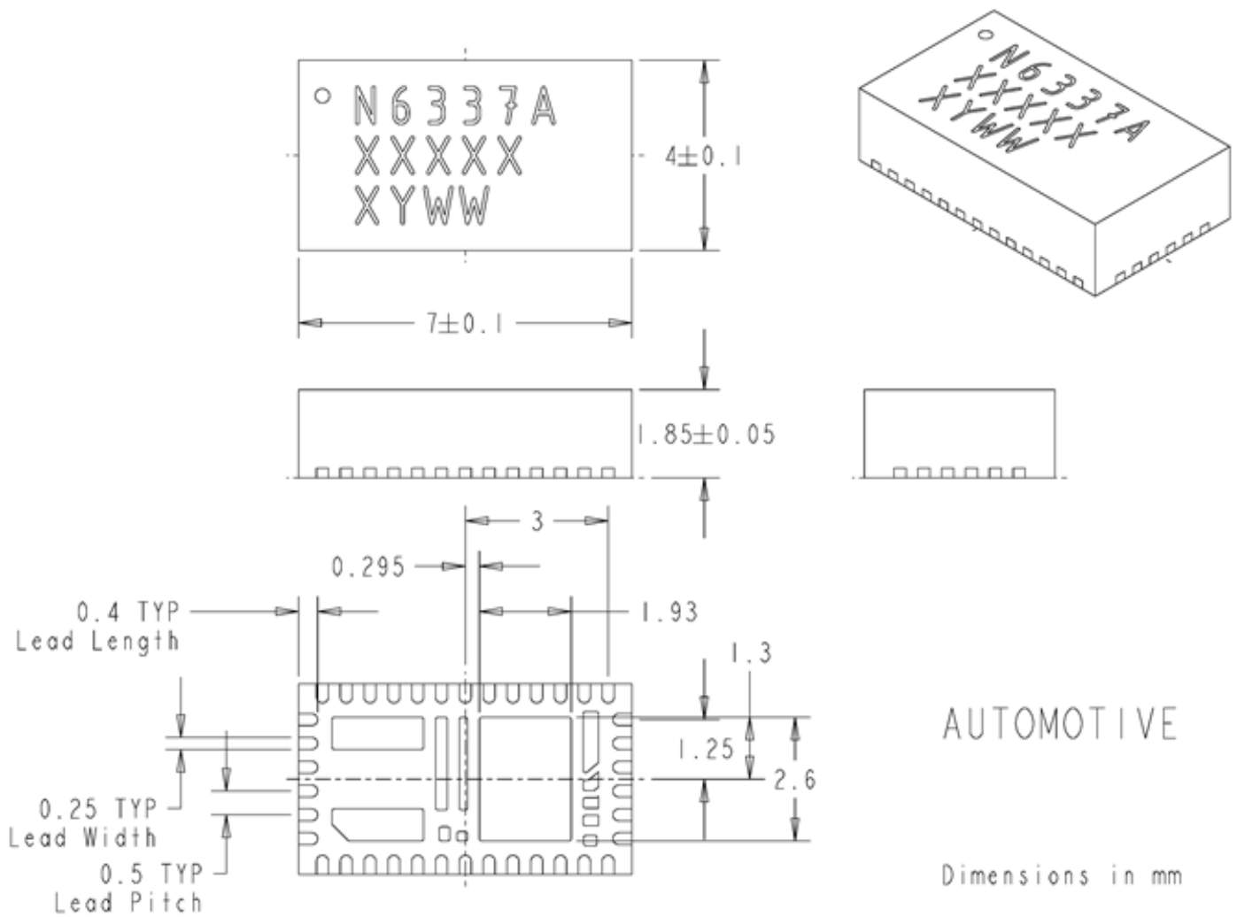
Figure 12: EN6337QA Package Dimensions
