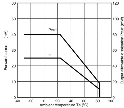
Fig 4. LED Current vs. Ambient Temperature Characteristics (Typical)
