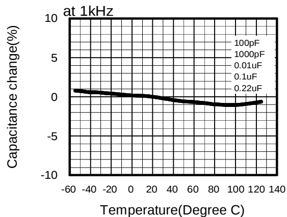
Temperature Characteristics
