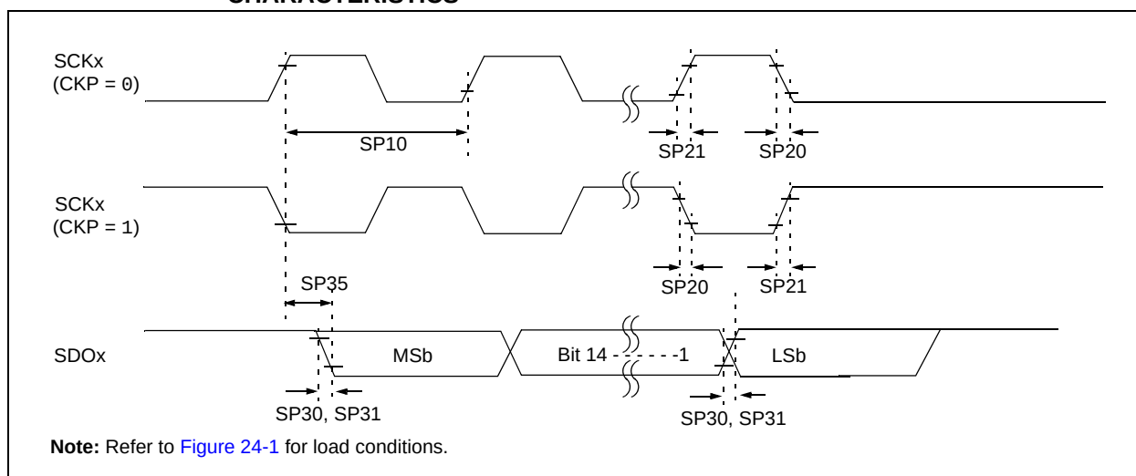
FIGURE 24-11: SPIx MASTER MODE (HALF-DUPLEX, TRANSMIT ONLY CKE = 0) TIMING CHARACTERISTICS
