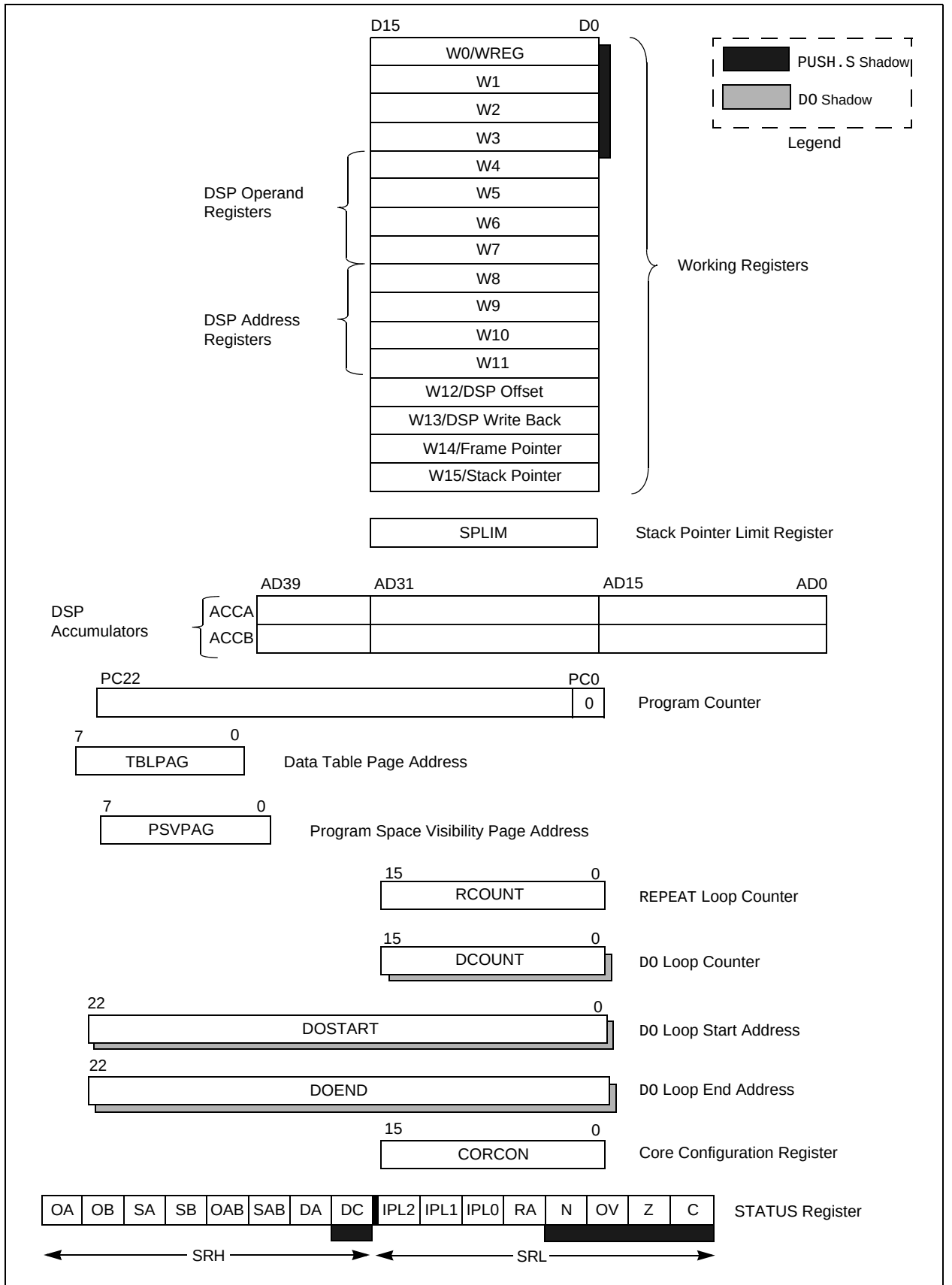
FIGURE 3-2: dsPIC33FJ06GS101/X02 and dsPIC33FJ16GSX02/X04 PROGRAMMER'S MODEL
