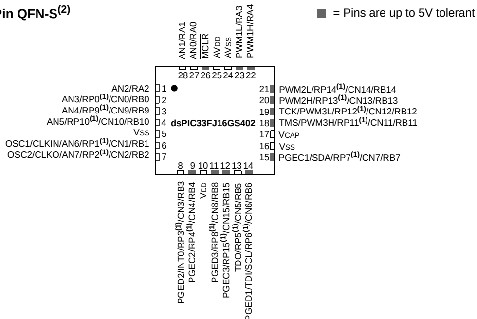
28-Pin QFN-S (2)
