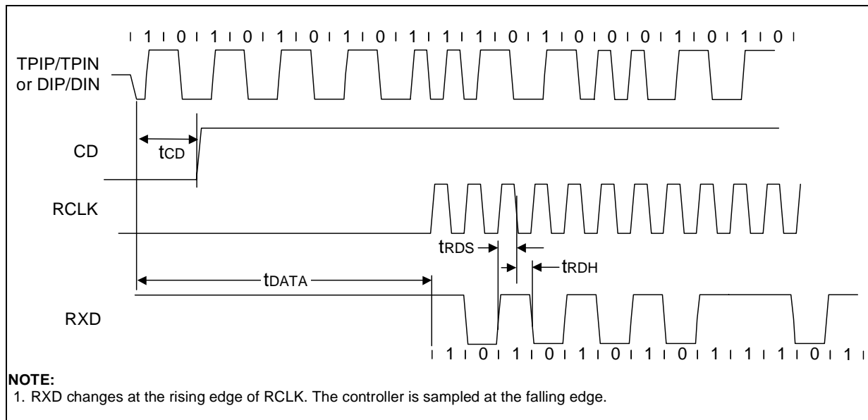
Figure 23. Mode 2 RCLK/Start-of-Frame Timing
