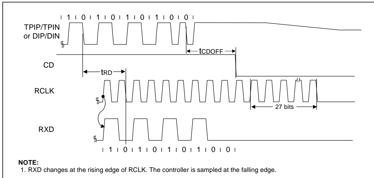
Figure 30. Mode 3 RCLK/End-of-Frame Timing (LXT901 only)
