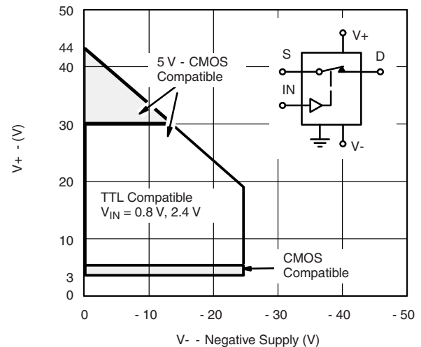
Operating Voltage
