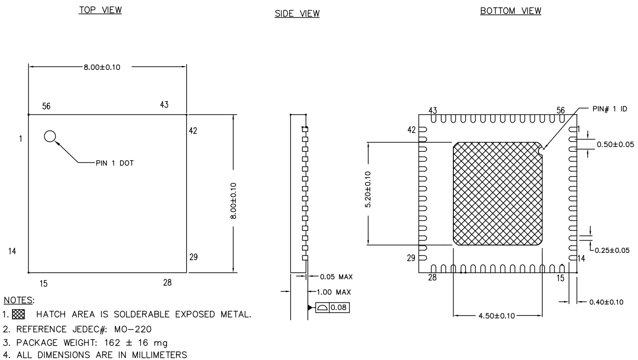
Figure 4. 56-pin QFN (8 × 8 × 0.9 mm) - Sawn
