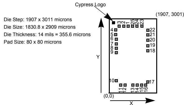
Figure 56. Die Form
