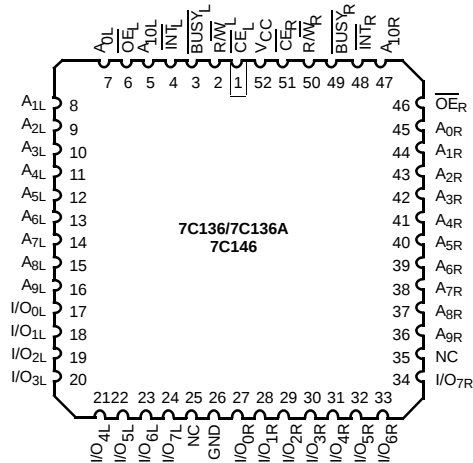
Figure 1. 52-Pin PLCC (Top View)
