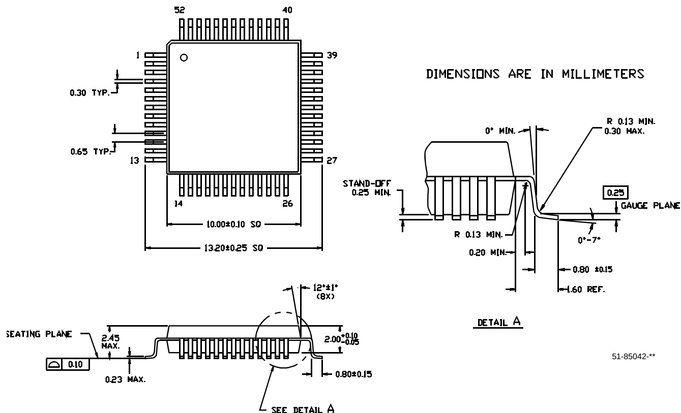
Figure 17. 52-Pin Pb-Free Plastic Quad Flatpack N52
