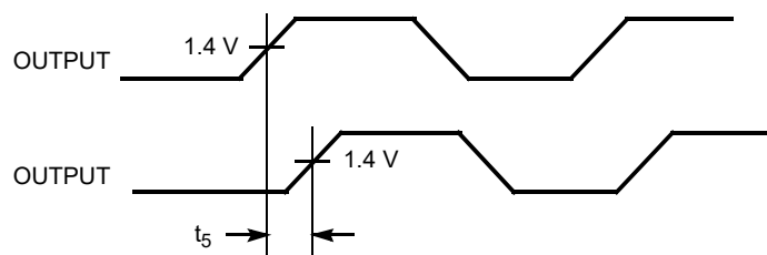
Figure 7. Output-Output Skew
