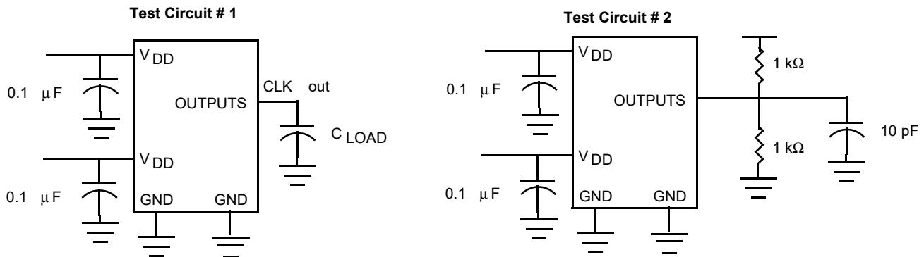
Figure 4. Test Circuits
