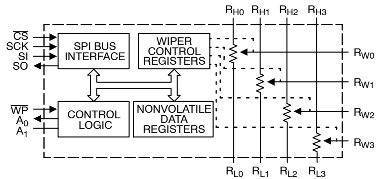
Figure 1. Functional Diagram
