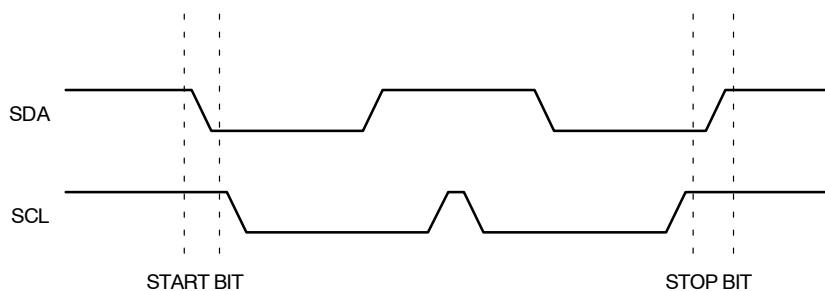
Figure 5. Start/Stop Timing
