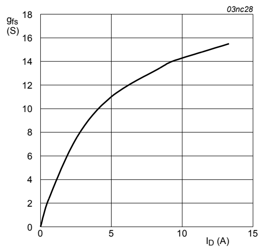
Fig. 8. Forward transconductance as a function of drain current; typical values T_j = 25^\circ\text{C}; V_{DS} = 25\text{V}
