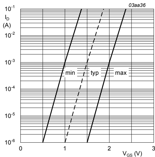
Fig. 7. Sub-threshold drain current as a function of gate-source voltage T_j = 25^\circ\text{C}; V_{DS} = 5\text{V}
