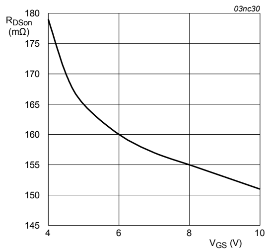
Fig. 6. Drain-source on-state resistance as a function of gate-source voltage; typical values T_j = 25^\circ\text{C}; I_D = 5\text{A}
