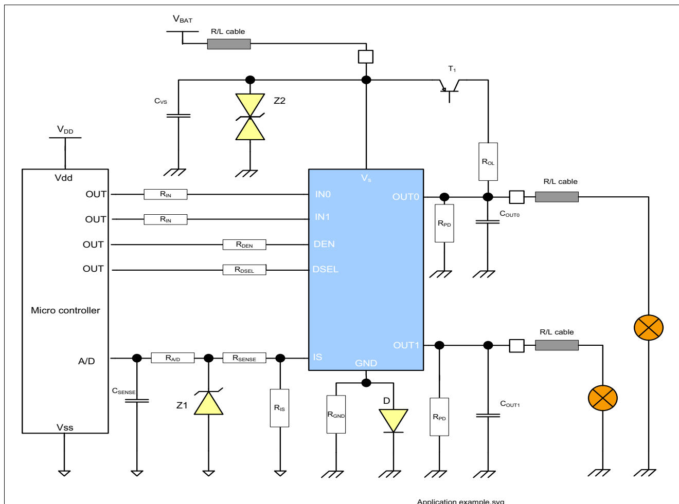
Figure 53 Application Diagram with BTS5120-2EKA
