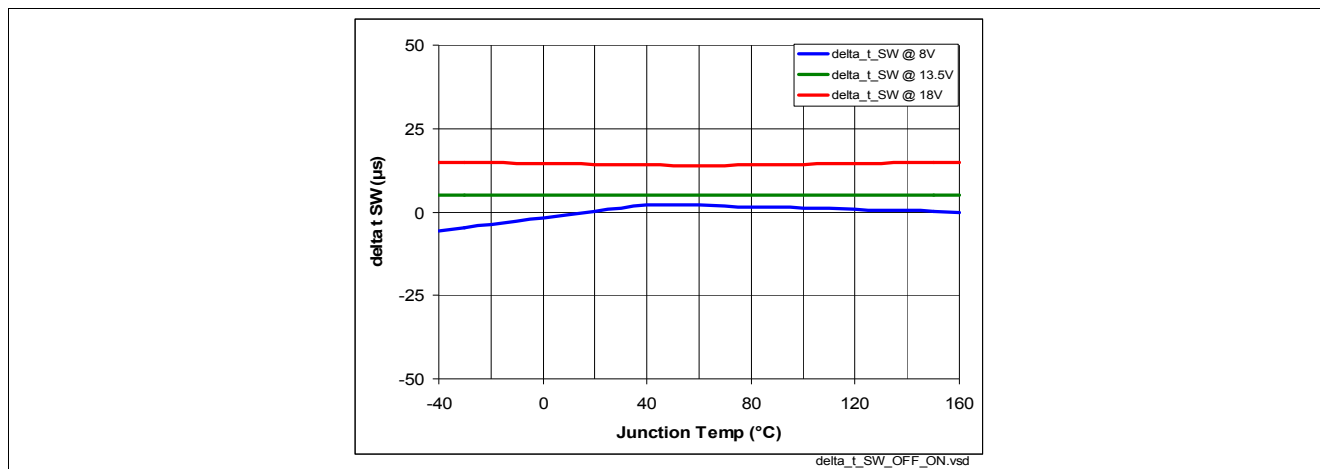
Figure 40 Turn ON / OFF matching \Delta t_{\text{SW}} = f(T_J; V_S) , R_L = 12 \Omega
