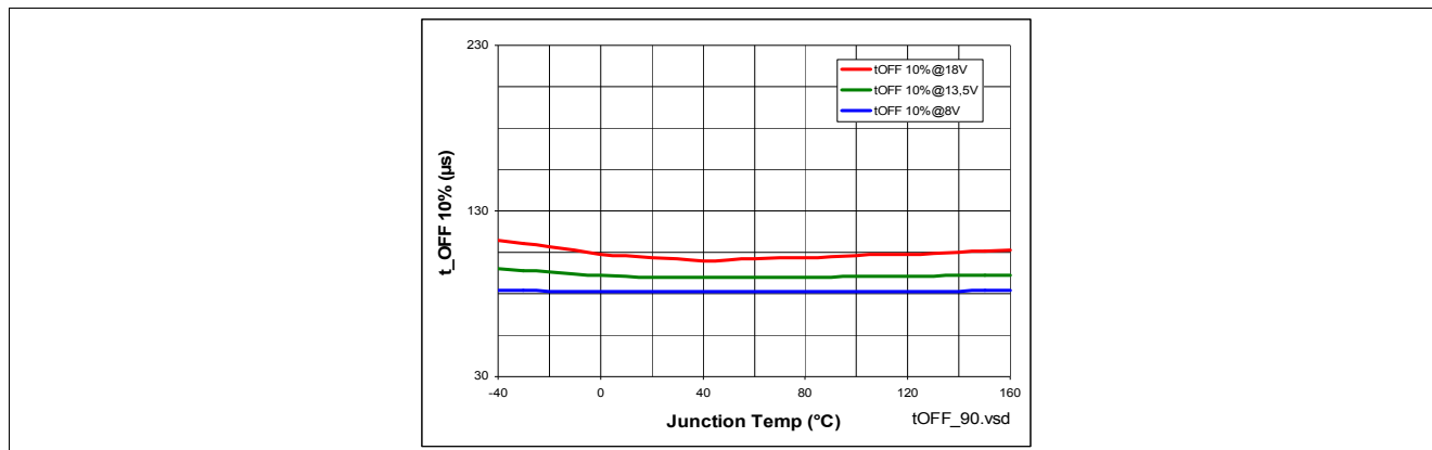
Figure 39 Turn OFF t_{\text{OFF}} = f(T_J; V_S) , R_L = 12 \Omega
