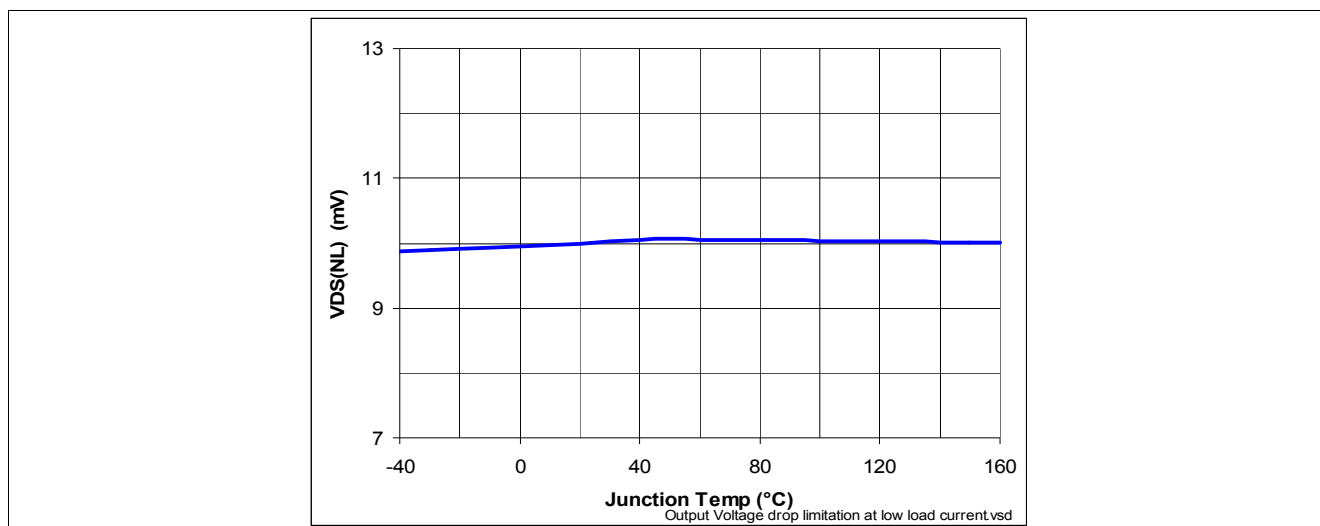
Figure 34 Output Voltage Drop Limitation at Low Load Current V_{DS(NL)} = f(T_J; V_S) ; I_L = I_{L(0)} = 30\text{mA}
