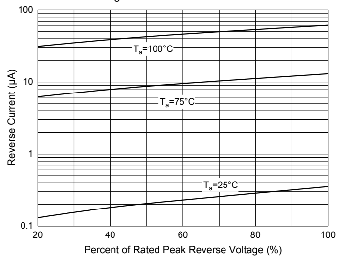
Fig. 2 - Reverse Characteristics
