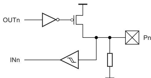
Figure 13-5. Output Configuration - Wired-OR with Optional Pull-down
