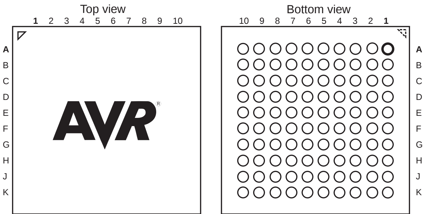
Figure 2-2. CBGA-pinout
