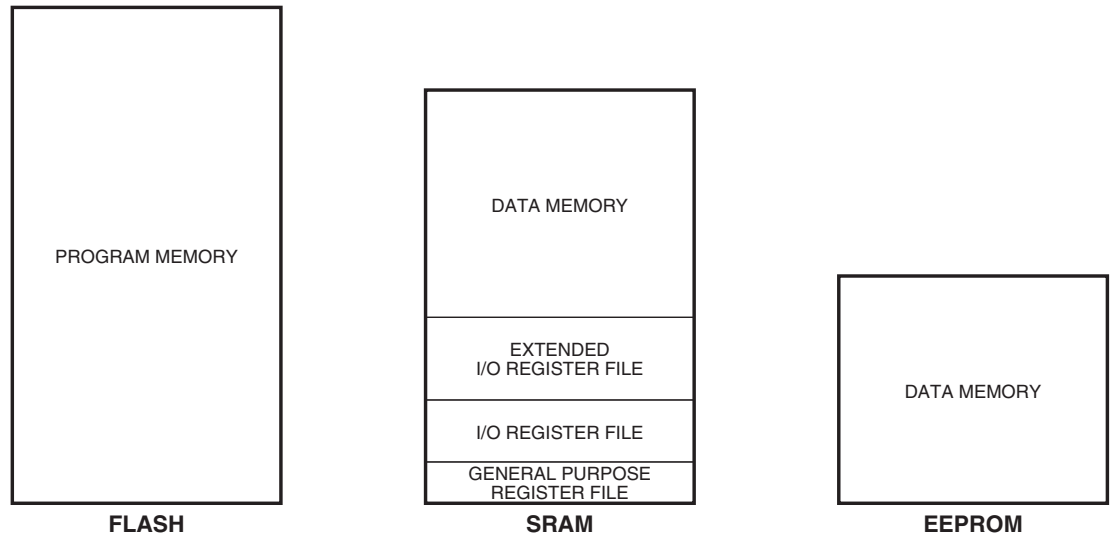
Figure 5-1. Memory Overview.
