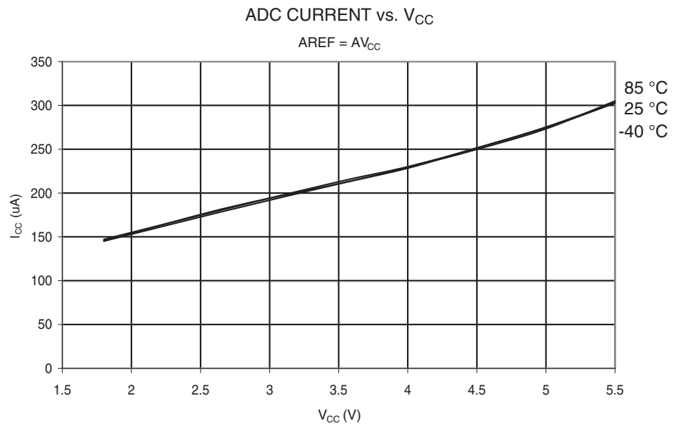
Figure 23-16. ADC Current vs. V_{CC} ( A_{REF} = A_{V_{CC}} )
