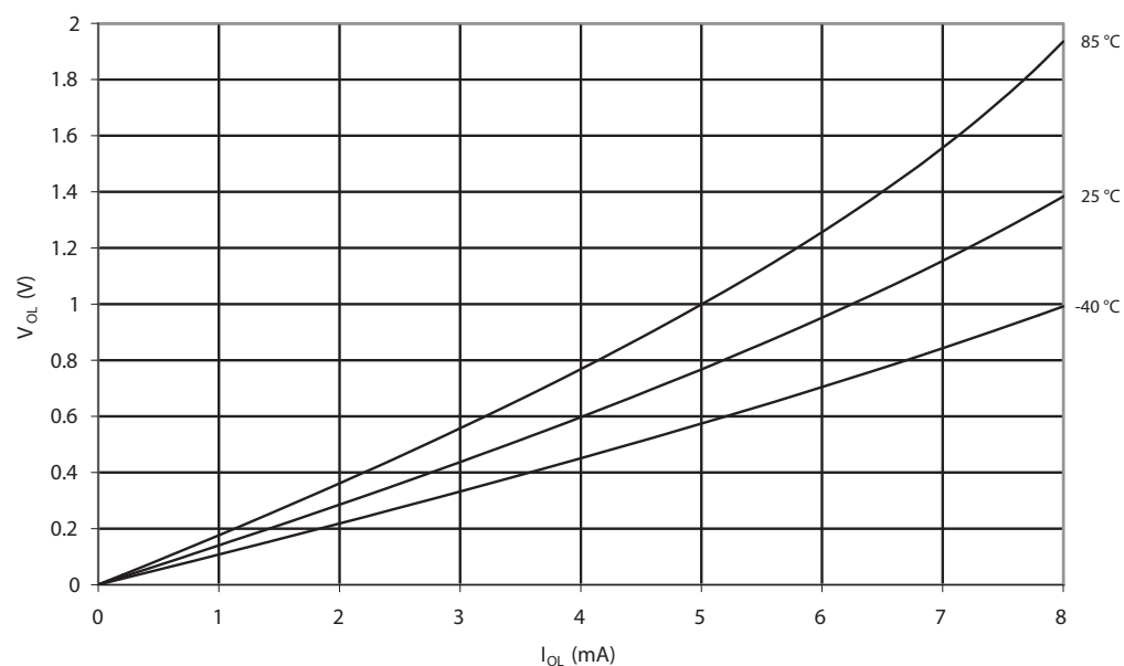
Figure 21-89. V_{OH} : Output Voltage vs. Source Current Reset Pin as I/O, V_{CC} = 3V
