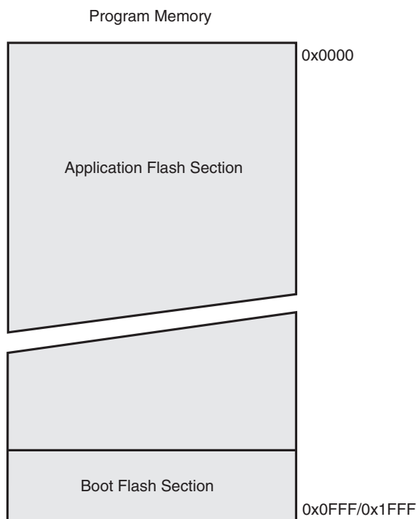
Figure 5-2. Program Memory Map, ATmega88 and ATmega168
