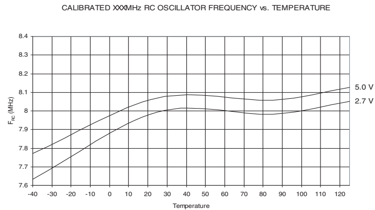
Figure 28-20. Calibrated 8 MHz RC Oscillator Frequency vs. Temperature
