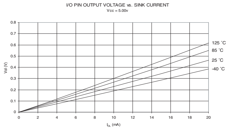
Figure 28-11. Output Low Voltage vs. Output Low Current ( V_{CC} = 5.0V )
