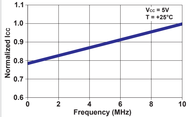
Figure 5-2. Normalized Supply Current vs. Address Frequency
