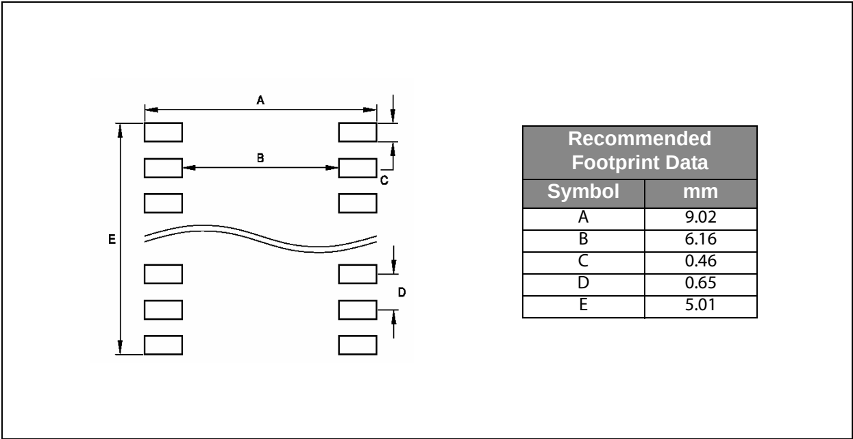
Figure 41: PCB Footprint
