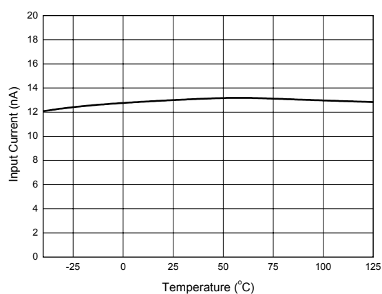
Figure 5. Input Current
