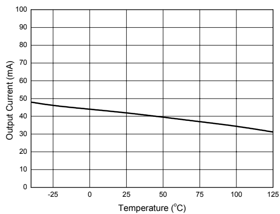
Figure 14. Current Limiting
