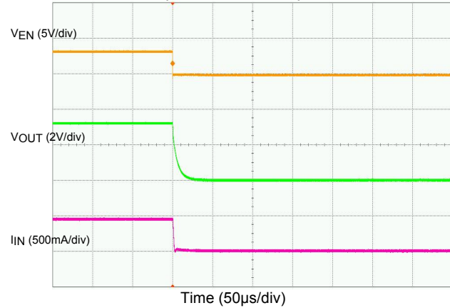
AP2281-3 Turn-Off ( V_{IN} = 3.3V , R_L = 7\Omega )
