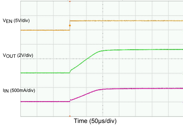
AP2281-3 Turn-On ( V_{IN} = 3.3V , R_L = 7\Omega )
