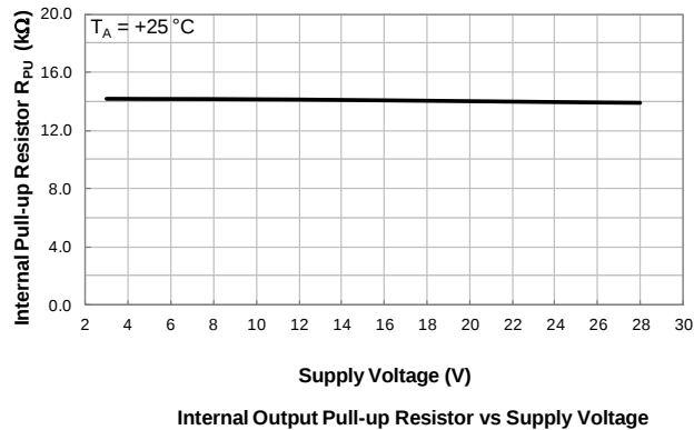
Internal Output Pull-up Resistor vs Supply Voltage
