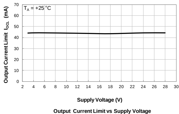
Output Current Limit vs Supply Voltage
