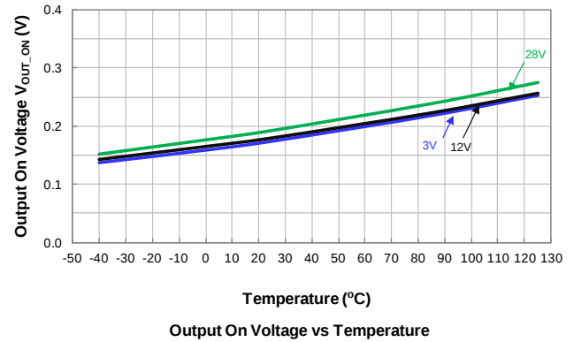
Output On Voltage vs Temperature
