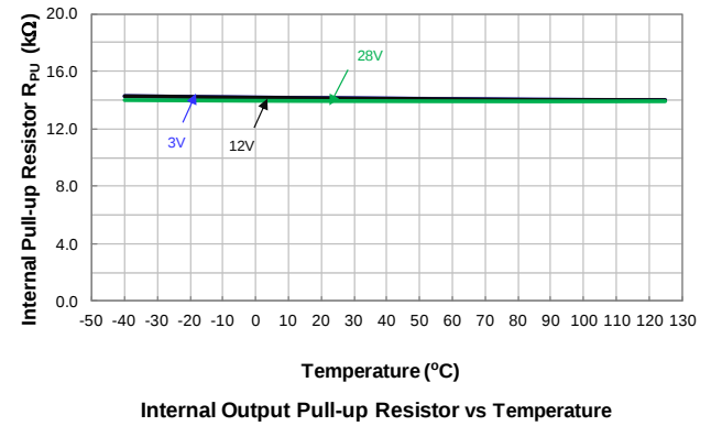
Internal Output Pull-up Resistor vs Temperature
