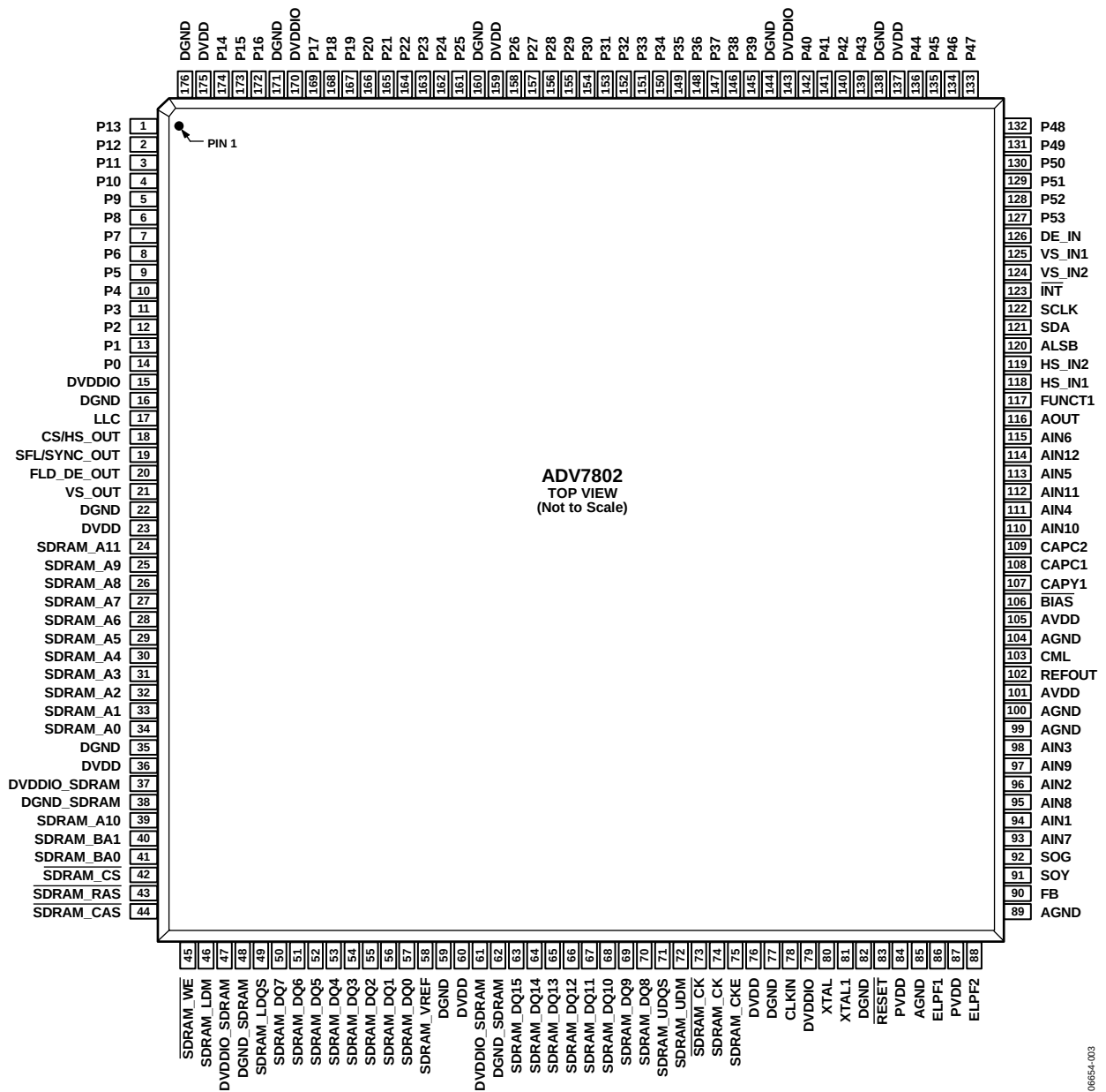
Figure 7. Pin Configuration
