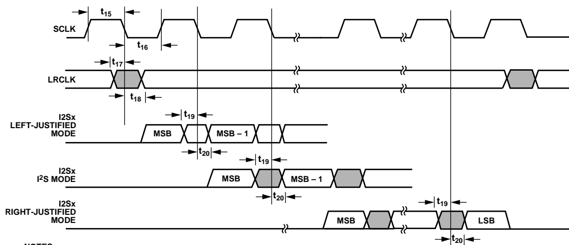
Figure 5. I²S Timing
