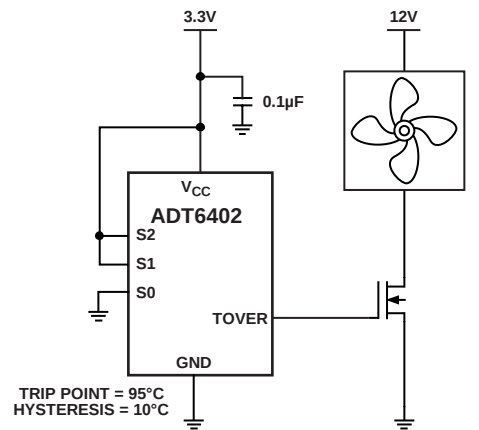
Figure 16. Overtemperature Fan Control
