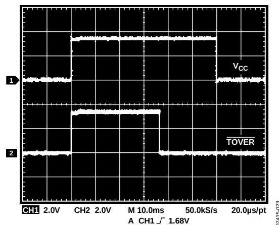
Figure 13. ADT6401 Start-Up Delay
