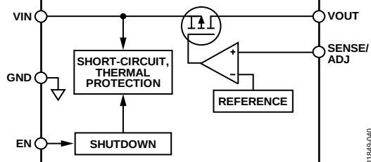
Figure 42. Internal Block Diagram
