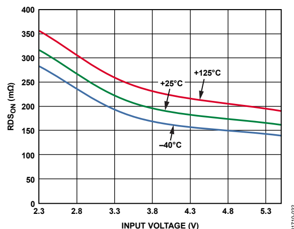
Figure 32. LFCSP NMOS R_{DS_{ON}} vs. Input Voltage Across Temperature
