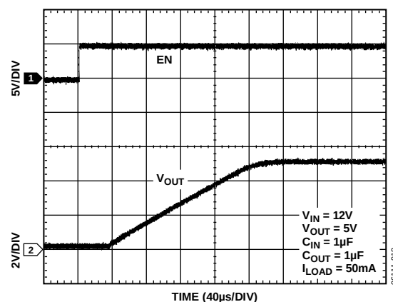
Figure 18. Start-Up Time
