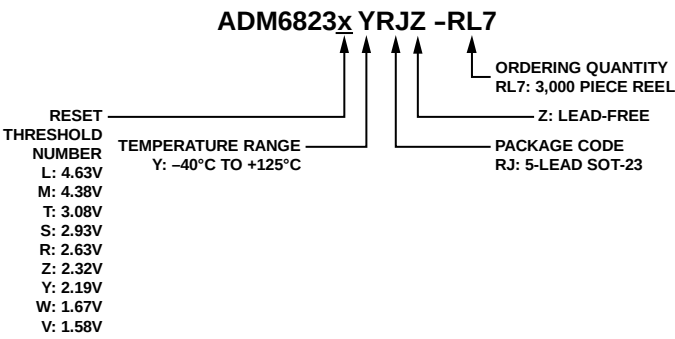
Figure 17. Ordering Code Structure
