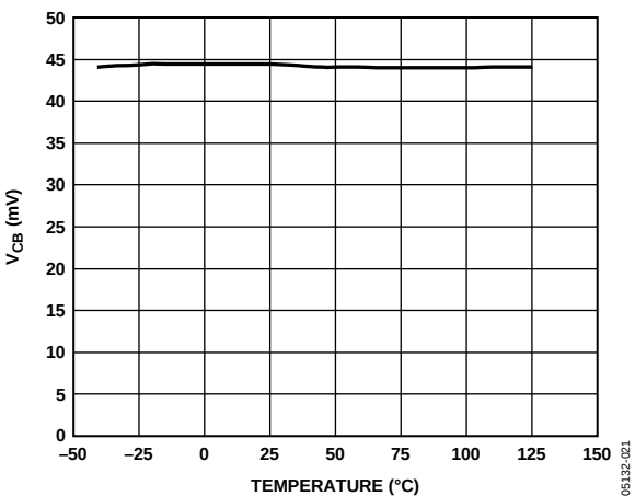
Figure 29. Cct Breaker Voltage vs. Temperature
