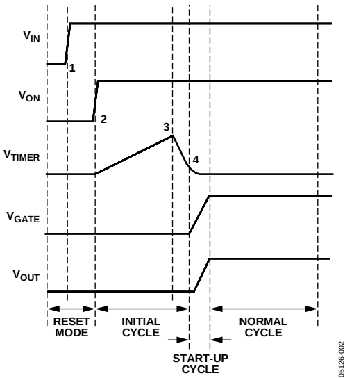
Figure 30. Power-Up Timing
