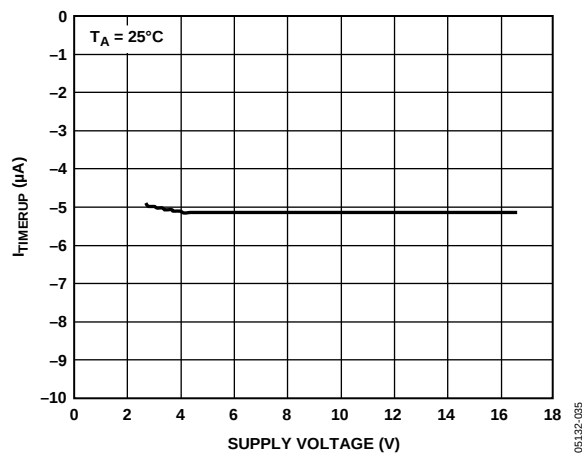
Figure 14. I_{TIMERUP} (in Initial Cycle) vs. Supply Voltage
